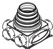
DB206 with stepped mass flow adapter 125 - 200 mm
